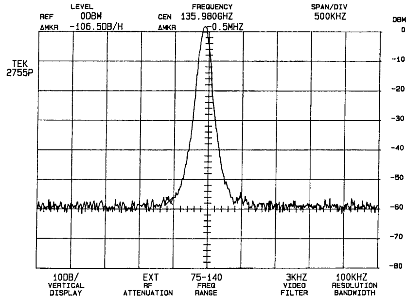
Fig. 3. Spectrum of the oscillator with device pair #1 of Table I. Power level: 130 mW, center frequency: 135.980 GHz, vertical scale: 10 dB/div, horizontal scale: 500 kHz/div, BW: 100 kHz, VBW: 3 kHz.
