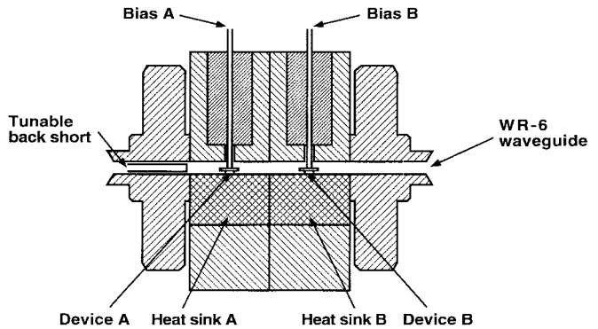
Fig. 1. Schematic of the in-line dual-cavity waveguide circuit for Gunn device power combining.
