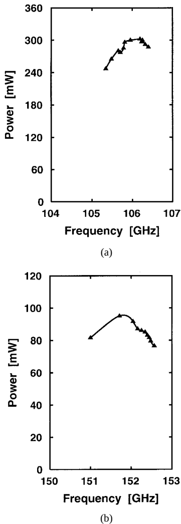
Fig. 4. Mechanical tuning characteristics of the power-combined device pairs (a) #3 and (b) #2 of Table I.
