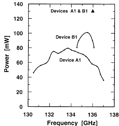
Fig. 2. Mechanical tuning characteristics of devices A and B of pair #1 in individual oscillators at 80% and 100% of the maximum dc bias, respectively.
